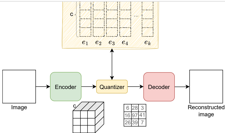
Figure 12: Image tokenizer training process
