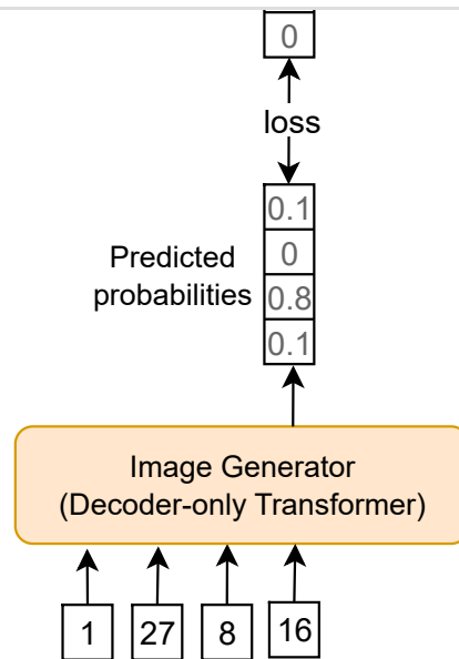
Figure 13: Image generator loss calculation
