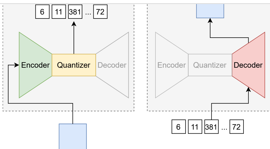
Figure 4: Image tokenizer's encoding and decoding
