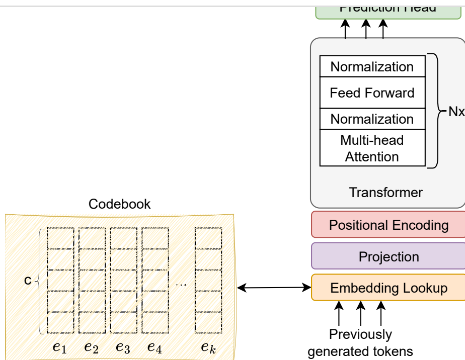
Figure 11: Decoder-only Transformer components
